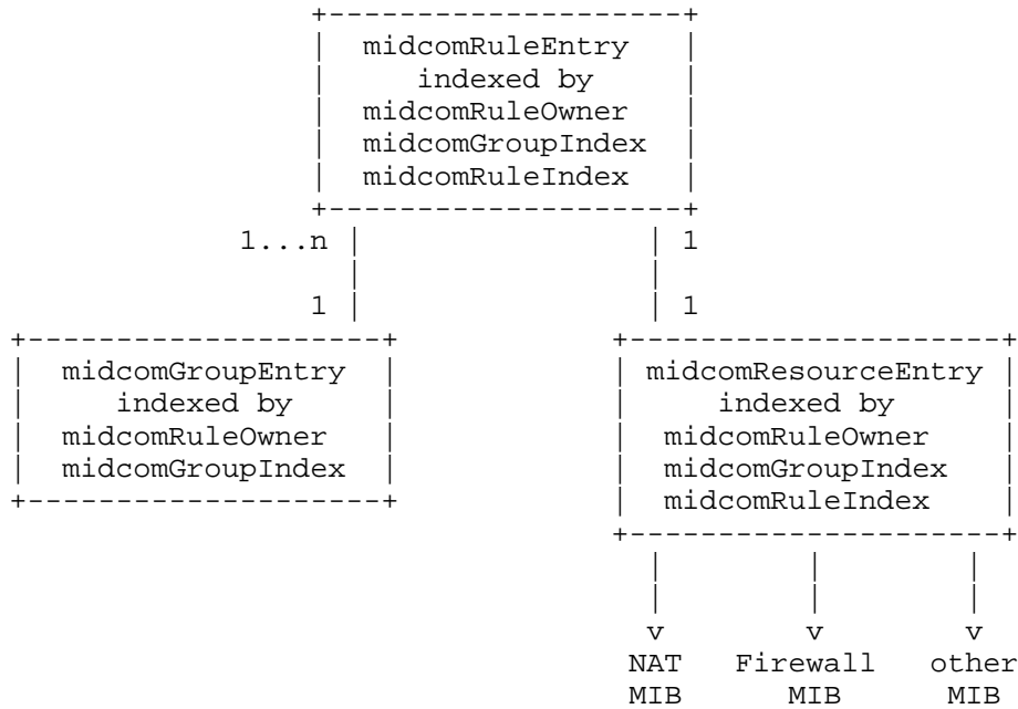
Figure 6: Entity relationships of table entries
